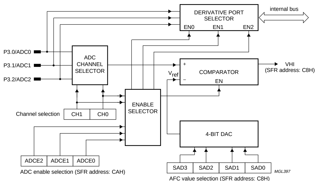
Fig.27 ADC block diagram.
